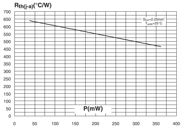
Fig. 9: Thermal resistance junction to ambient versus power dissipation (epoxy printed circuit board FR4, e CU =35μm, typical values).
